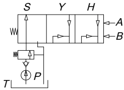
HİDROLİK SEMBOL HYDRAULIC SYMBOL
